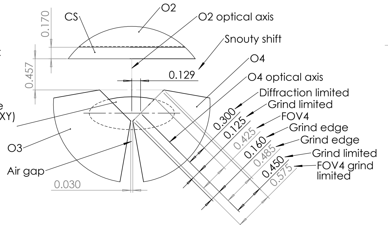
DETAIL C SCALE 30 : 1
