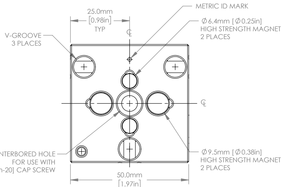
BOTTOM PLATE (KBB50/M) TOP VIEW
