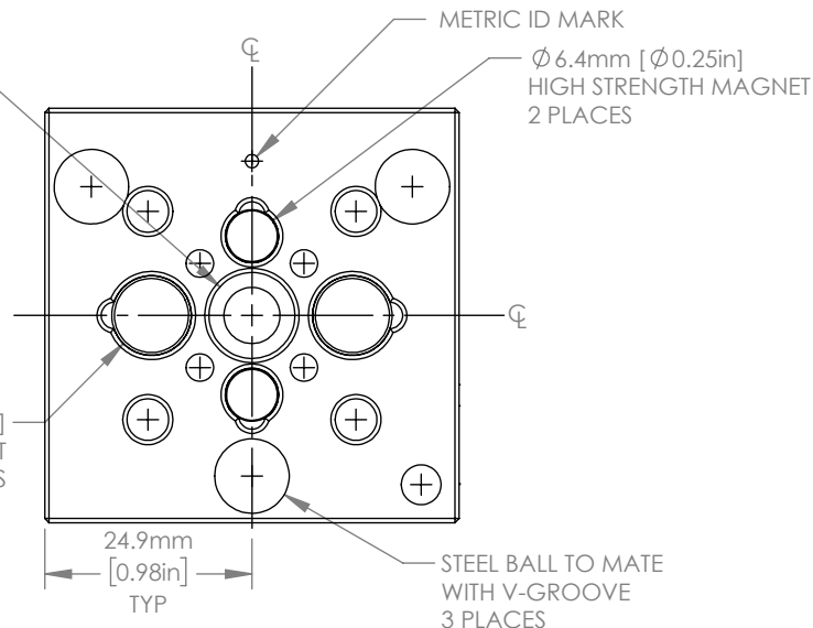
TOP PLATE (KBT50/M) BOTTOM VIEW
